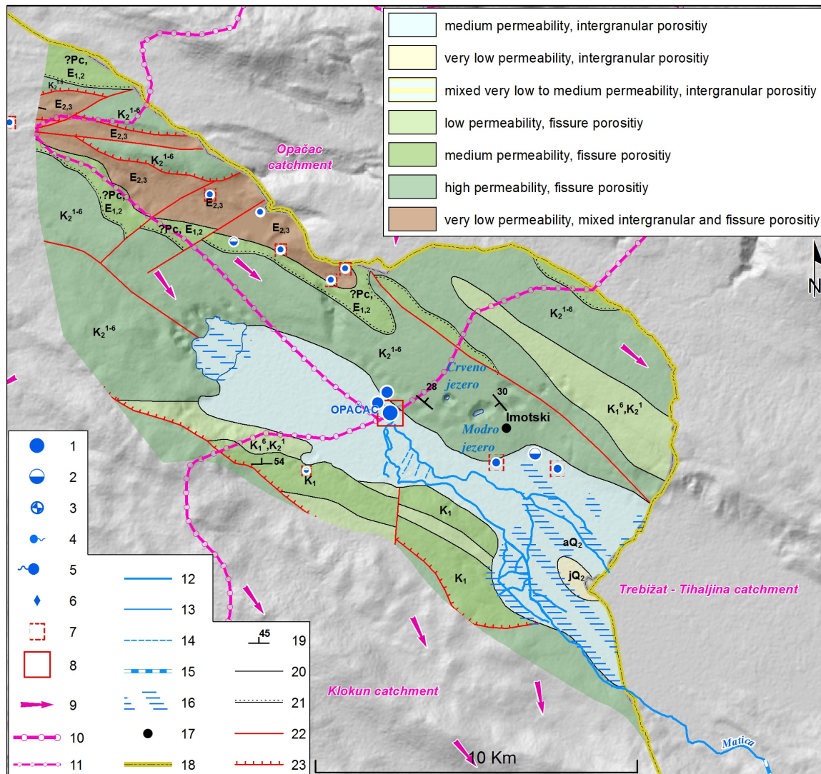
Figure 9. Hydrogeological map of the catchment area of the Imotsko polje springs. Legend: 1 constant spring 2 occasional spring 3 estavelle 4,5 springs of different abundance 7 primitive catchment 8 public water supply site 9 groundwater flow 10 watershed 11 presumed watershed 12-14 surface flow 16 flood area, wetland 17 settlement 18 state border 19 layer position 20 Normal lithostratigraphic boundary 21 erosion-discordant geological boundary 22 normal fault 23 reversal fault
